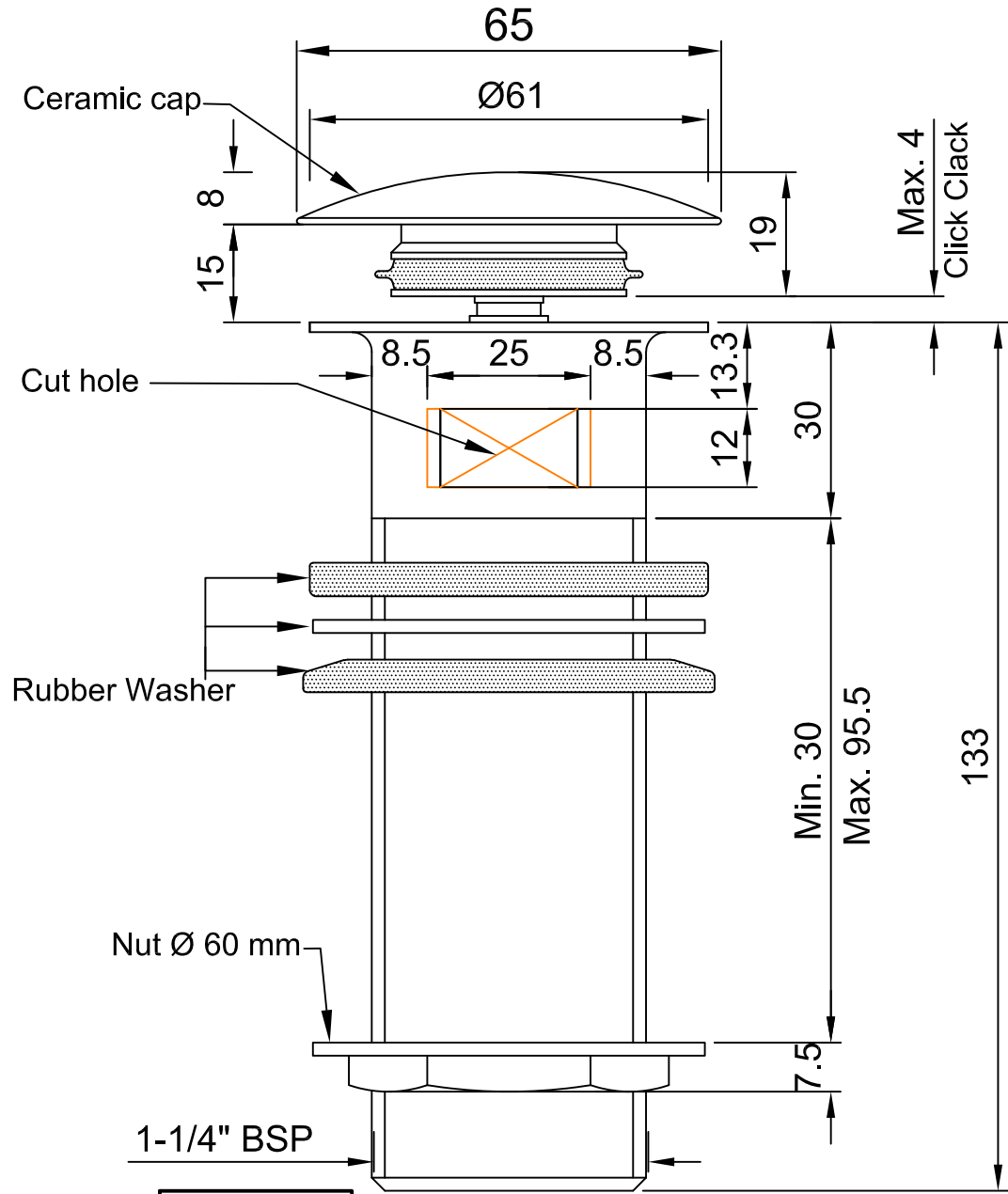
SIDE VIEW
